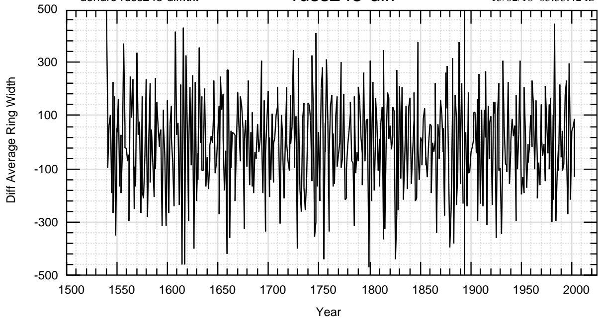
dendro russ243 Diff
