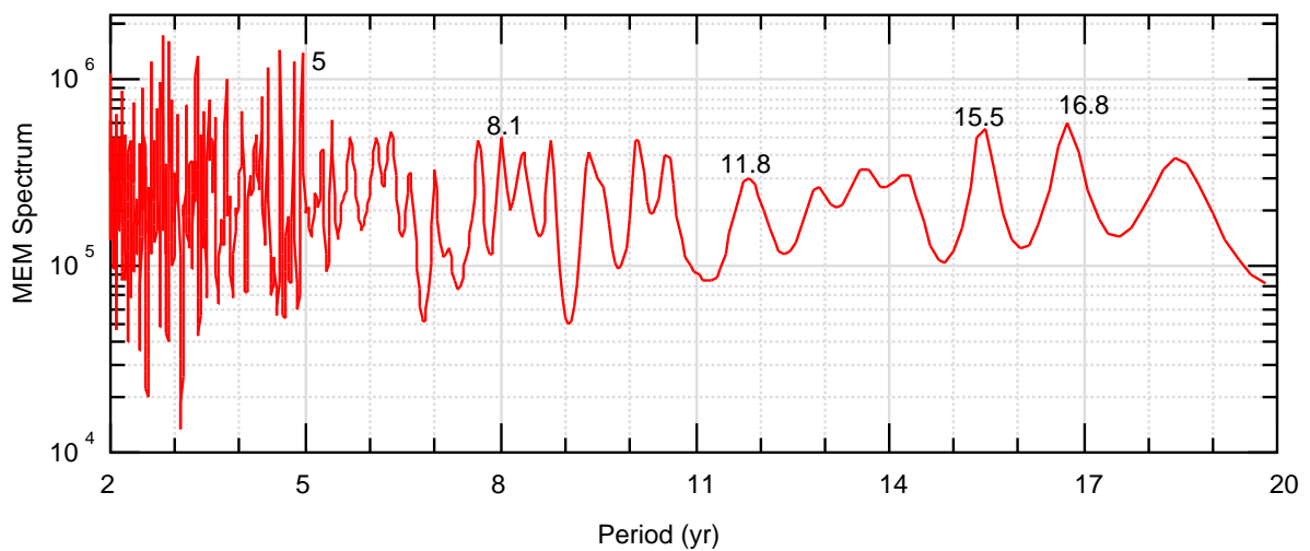
dendro russ243 Diff
