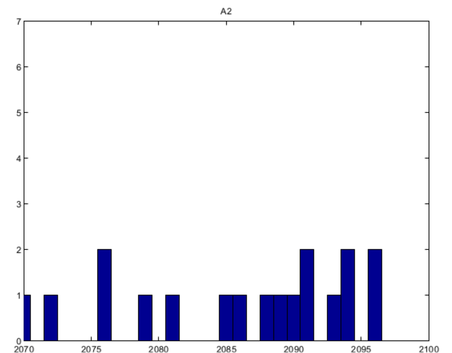
Figure 5.6: Number of medicanes per season in the A2 simulation.
