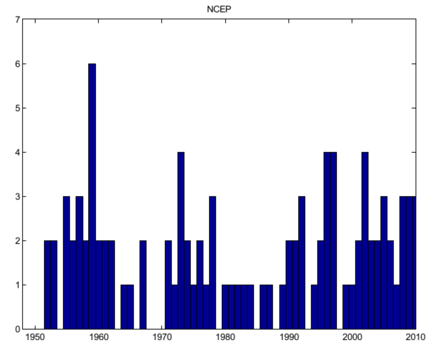
Figure 4.3: Number of medicanes per season in the NCEP60 simulation.
