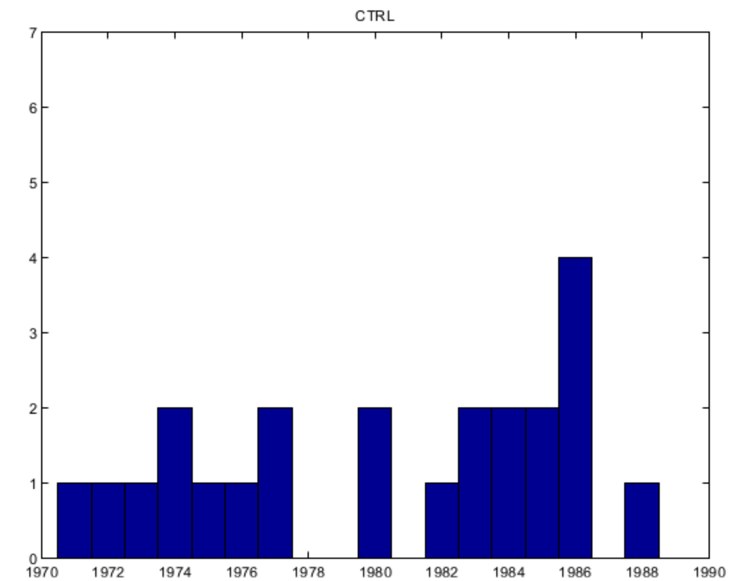
Figure 5.3: Number of medicanes per season in the C20 simulation.
